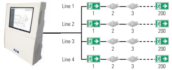
CGLine+ Web Touchscreen Controller
