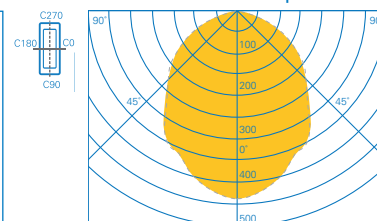
BeamTech 1 Light Head Wide beam at 0° slope
