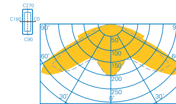
Escape route illumination with symmetric optics
