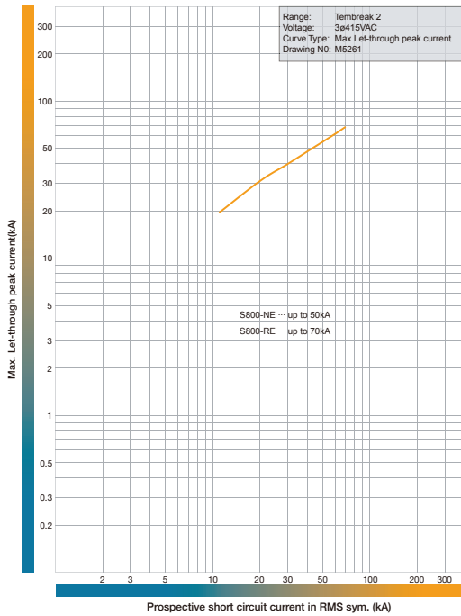
Let-Through Peak Current Characteristics S800-NE, S800-RE. 415V AC.
