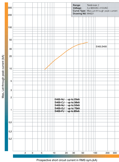
Let-Through Peak Current Characteristics E400-NJ, S400-CJ, S400-NJ, S400-GJ, S400-PJ. 415V AC.
