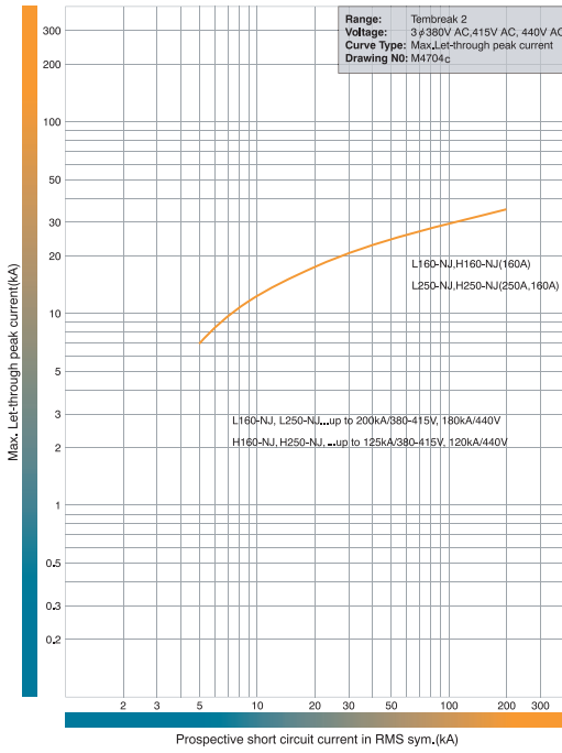
Let-Through Peak Current Characteristics H160-NJ, L160-NJ, H250-NJ. 380/415/440V AC.
