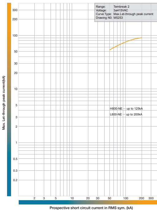
Let-Through Peak Current Characteristics H800-NE, L800-NE. 415V AC.
