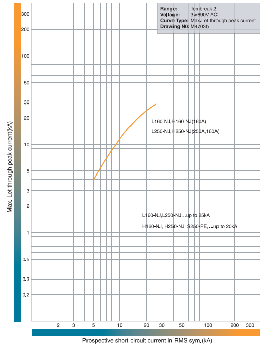
Let-Through Peak Current Characteristics H160-NJ, L160-NJ, H250-NJ, L250-NJ. 690V AC.
