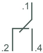
Terminal Designations and Function of General Purpose Auxiliary Switch
