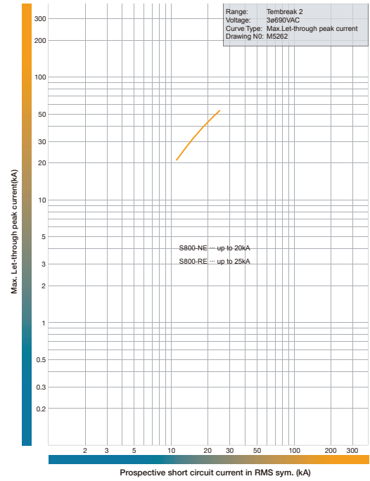
Let-Through Peak Current Characteristics S800-NE, S800-RE. 690V AC.
