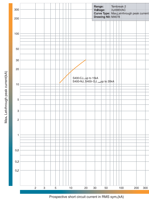
Let-Through Peak Current Characteristics S400-CJ, S400-NJ, S400-GJ, S400-PJ. 690V AC.
