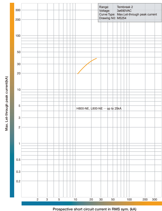
Let-Through Peak Current Characteristics H800-NE, L800-NE. 690V AC.
