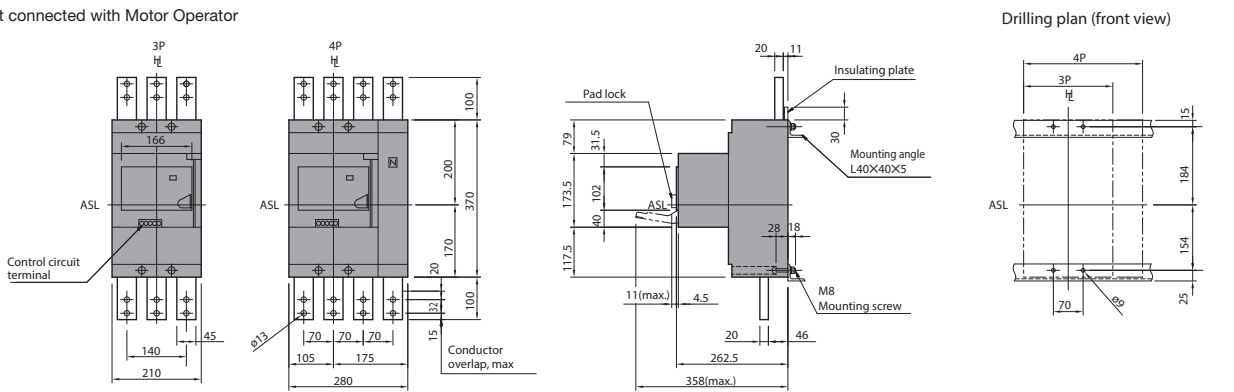
Rear connected with Motor Operator
