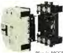
Plug-in MCCB and base
