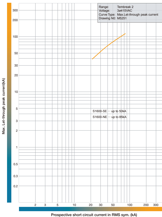
Let-Through Peak Current Characteristics S1600-SE, S1600-NE. 415V A
