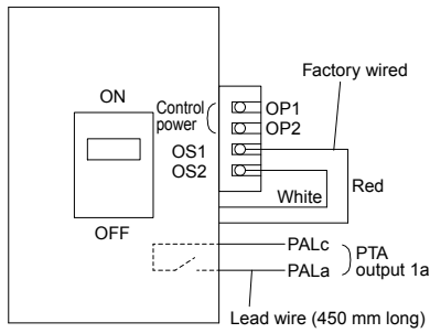
OCR power supply installed on the breaker
