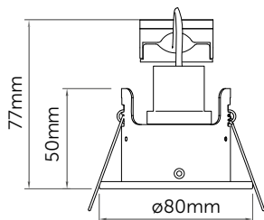
Fixed Downlight
