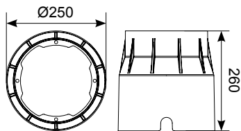
Installation Sleeve
