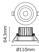
Cut out: Ø90-95mm
