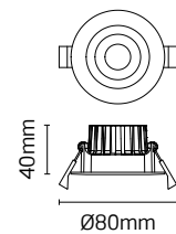
Cut out: Ø68-75mm
