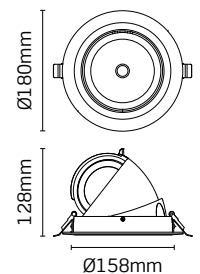
Cut out: Ø165-170mm
