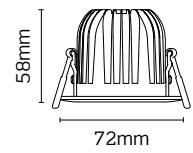
Cut out: Ø64mm
