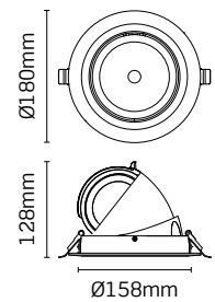
Cut out: Ø165-170mm
