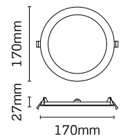
Cut out: Ø150-160mm
