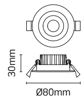
Cut out: Ø90-95mm
