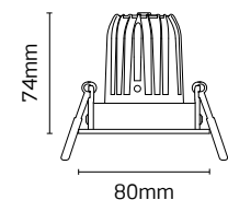
Cut out: Ø75mm
