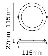
Cut out: Ø100-110mm
