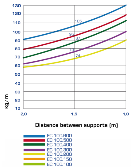
SAFE WORKLOAD - EASYCONNECT 100
