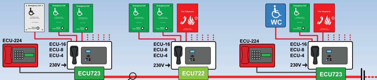
Networked SigTEL system wiring with multiple ECU-224 Desk Controllers connected
