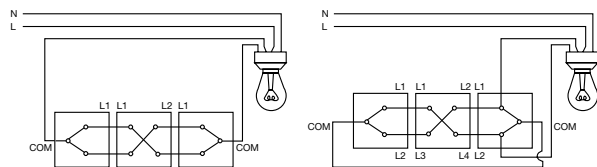
Diagram C – Intermediate circuits
