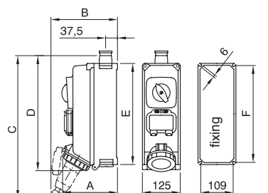
IP67 Watertight - Tais switched and interlocked socket with 4 modules window
