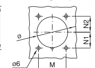
Drilling template
