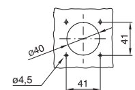
Drilling template
