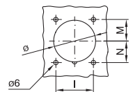
Drilling template
