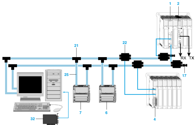
Network with PC cards for Modbus Plus
