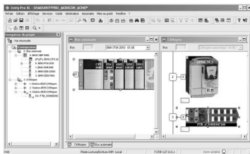
Graphical configuration of devices on CANopen bus
