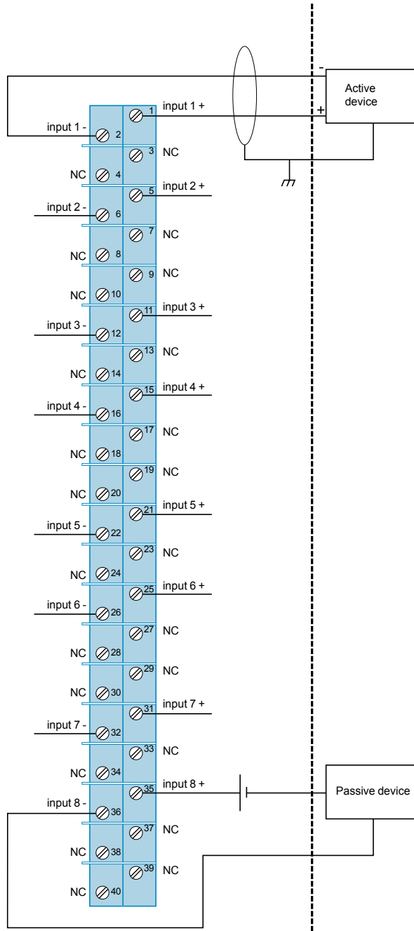
Connections for the safety analog input module 140 SAI 940 00S, 8 analog inputs
