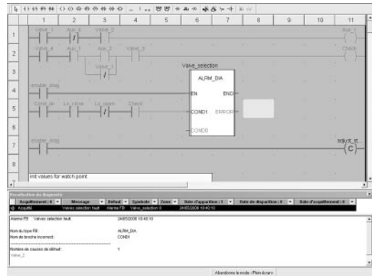
Diagnostics with fault cause analysis
