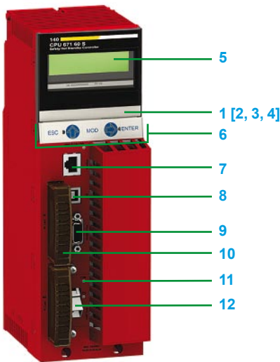
140 CPU 671 60S
