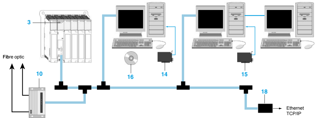
Network with PC cards for Modbus Plus
