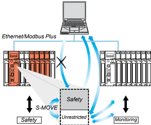
Only the S-MOVE function block is capable of reading in the unrestricted memory area.
