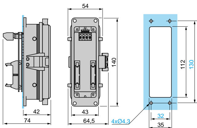
ABE 7ACC84
