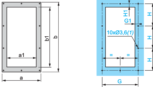
Cut-outs and drill holes
