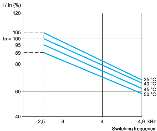
ATV 61EXS5C25N, ATV 61EXS5C31Y
