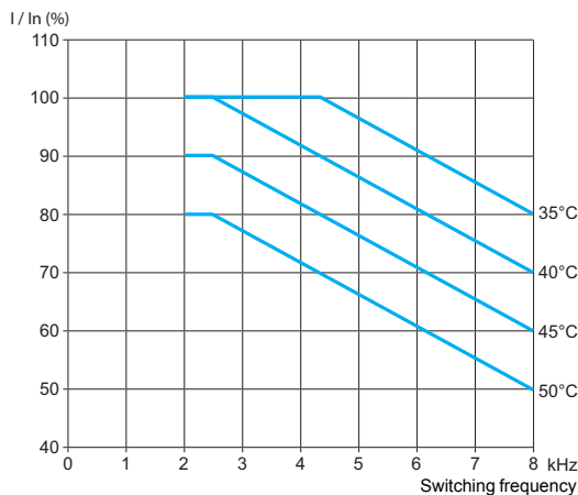
ATV 61EXC•C11N, ATV 61EXC•C13Y
