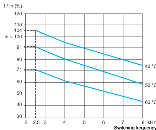
ATV 61HC31N4 combined with a 315 kW motor
