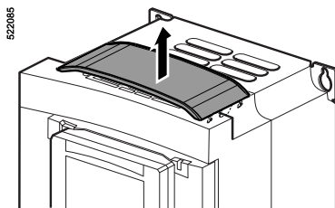
522085 Removing the protective blanking cover from: ATV 61H●●●M3, ATV 61HD11M3X, HD15M3X, ATV 61H075N4...HD18N4
