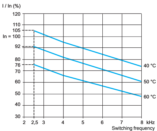
ATV 61HC31N4 combined with a 280 kW motor
