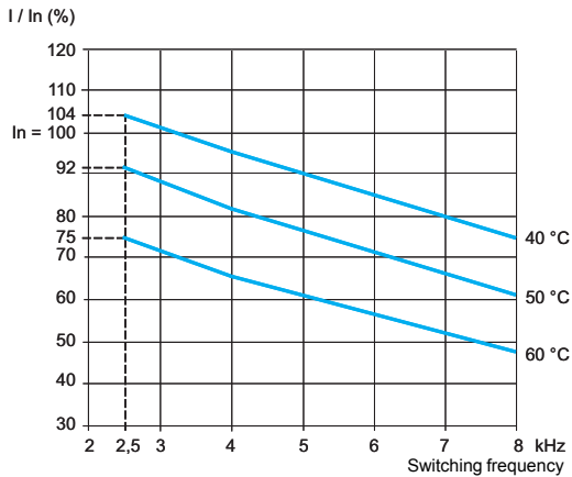
ATV 61HC22N4 combined with a 220 kW motor
