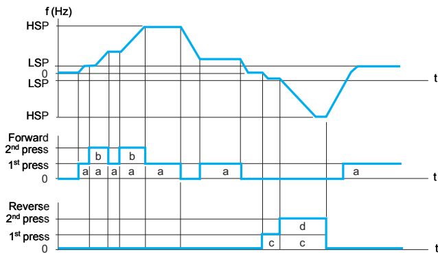
Example with double-action buttons and 1 logic input
