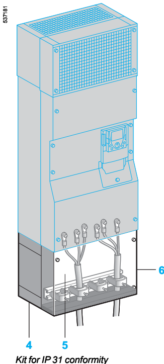
Kit for IP 31 conformity
