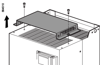
564510 Removing the protective blanking cover from: ATV 61HD18M3X...HD45M3X, ATV 61HD22N4...HD75N4, ATV 61HU30Y...HD90Y
