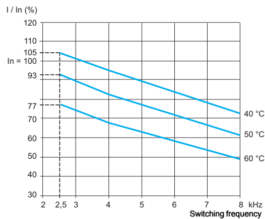
ATV 61HC63N4 combined with a 560 kW motor
