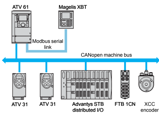
Independent machine with CANopen machine bus
