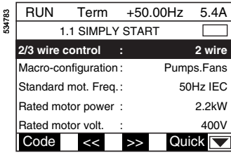
Simply Start menu
