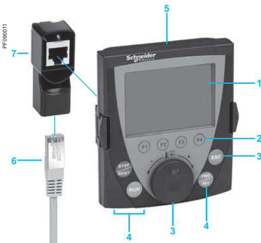
Graphic display terminal + female/female RJ45 adaptor + remote cable
