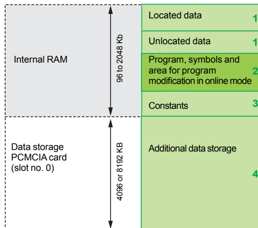
Processor with data storage memory card in slot no. 0
