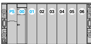
Extension rack address n with double-format power supply
