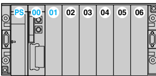
Primary rack address 0 with standard-format power supply and processor
