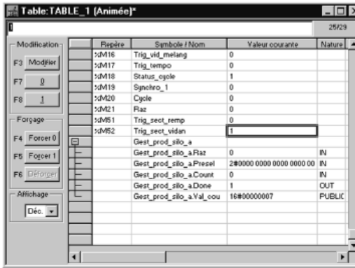
Animation table
