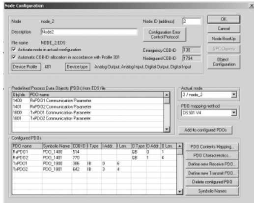
Example of SyCon device configuration screen
