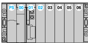
Primary rack address 0 with double-format power supply and standard-format processor
