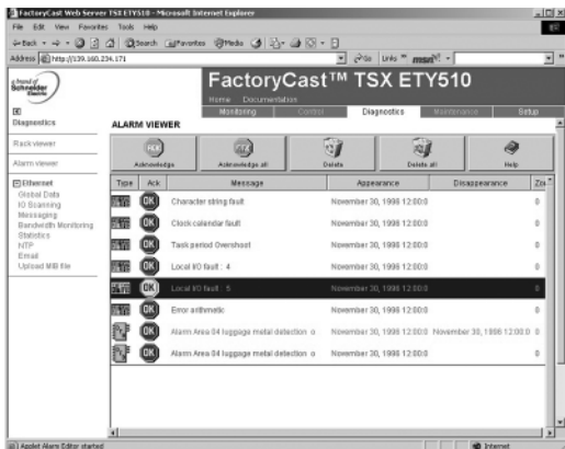
Alarm Viewer
