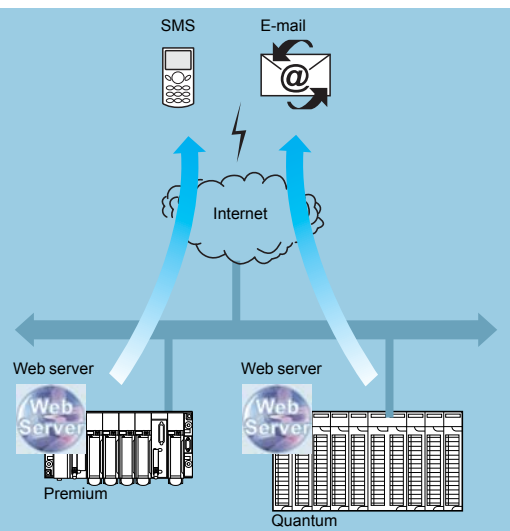
E-mail transmission
