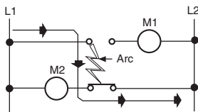
Figure 7—Contacts connected to opposite polarities. Line to line short (bold line) can occur through arc drawn when contacts operate
