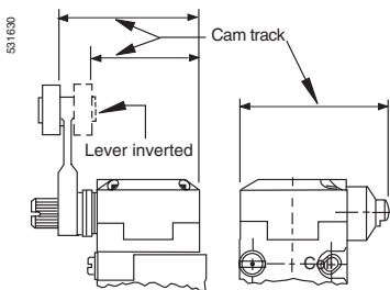
Figure 4—Cam track dimension
