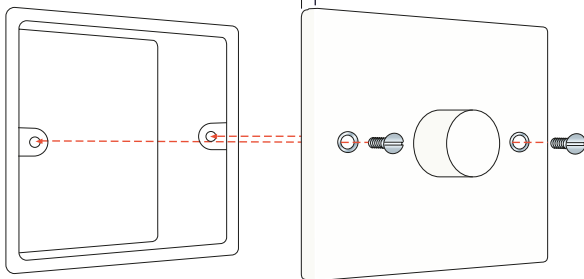
Box-Fix to Back Box
