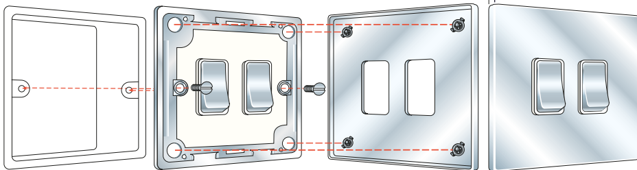
Screw fixings to Back Box
