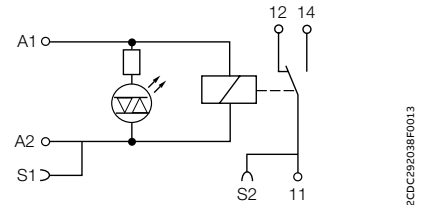
RB(R)121-12VDC/24VDC
