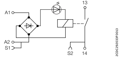
RB111-115VUC/230VUC
