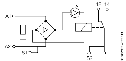
RB(R)121R-115VUC/230VUC
