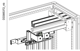
LVS04635 Connection to 5 mm Thick Horizontal Busbar
