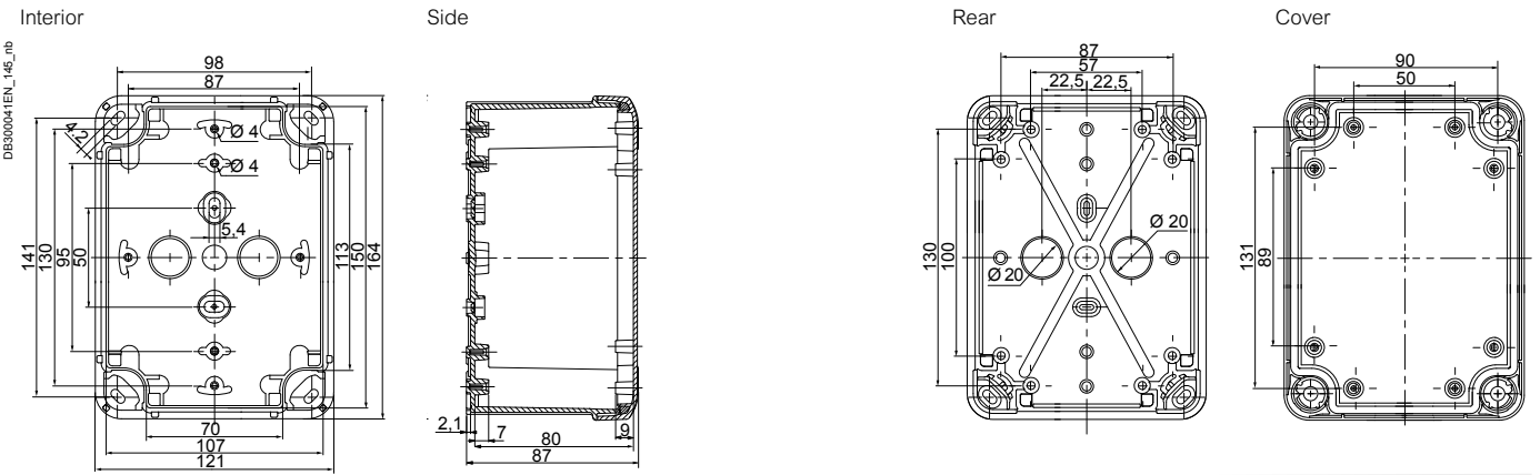
Box of 192 x 121 x 87 or 105 mm (external dimensions) NSYTB●●●19128 or NSYTB●●●191210
