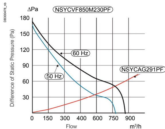
Flow Curves
