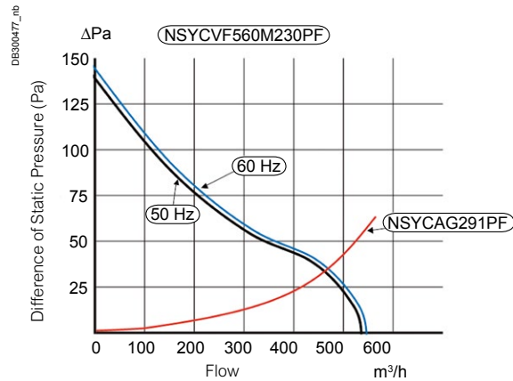
Flow Curves
