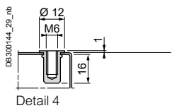
4 Crimped Blind Nuts for Direct Fixing of the Fixing Lugs
