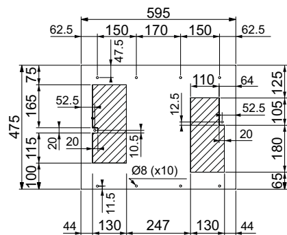
Internal Mounting Cut-Out
