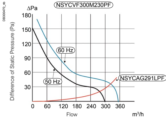
Flow Curves
