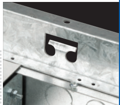
Rapid fit push lock secures base in floor aperture
