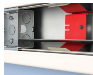
The rolled edge on the trunking opening and divider reduces the risk of injury or damage to cables when installing the trunking
