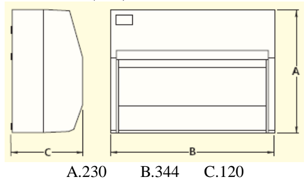
*Image depicts a 13 way unit*
