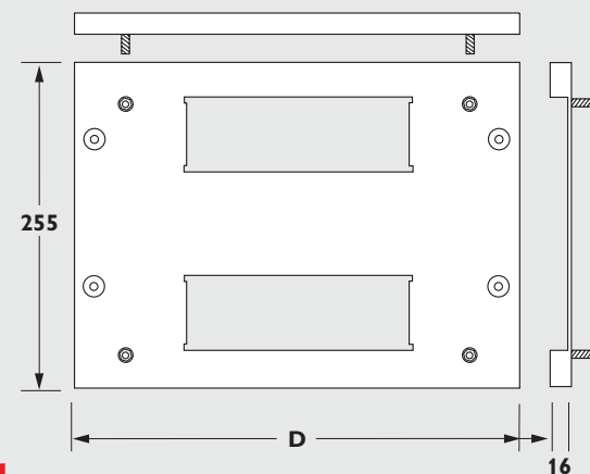
LEFT/RIGHT CABLE ENTRY PATTERNS
