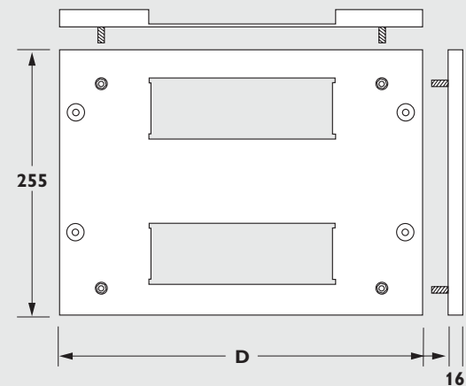
TOP/BOTTOM CABLE ENTRY PATTERNS
