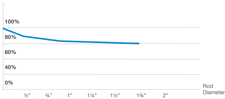
Effect of electrode diameter on resistance
