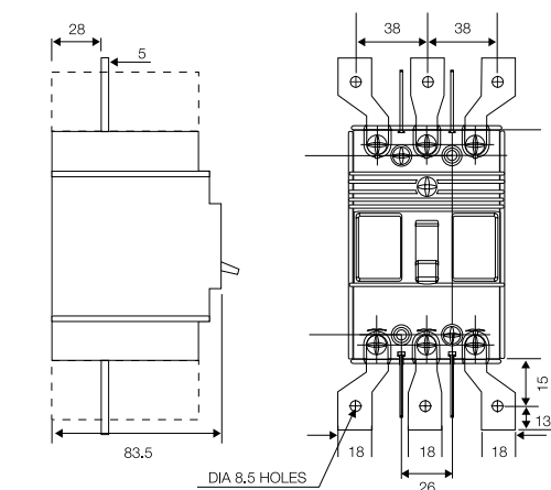
Three Pole with Extended Terminals
