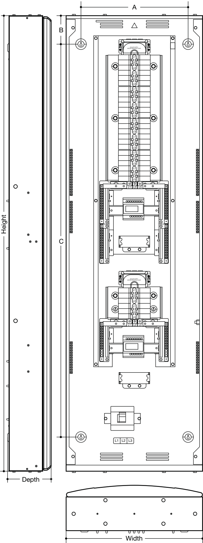
125A Rated Metered Boards
