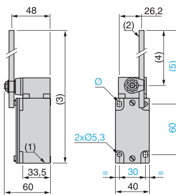
XCKJ•0559 ZCKJ• + ZCKE05 + ZCKY59
