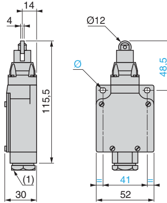
XCKL•06 ZCKL• + ZCKD06 ZCKLD3• + ZCKD06
